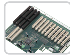
Flexible board configuration between industrial motherboard (IPPC-7157A) or passive backplane (IPPC-7158B)
